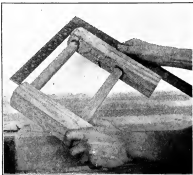
Fig. 222—Testing with Framing Square
